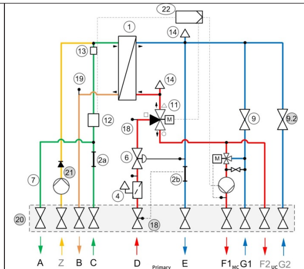
LogoMatic G2 MC-UC DHWC (Unmixed & mixed heating circuit as well as domestic hot water circulation)
