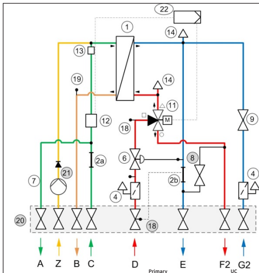
LogoMatic G2 UC DHWC (Unmixed heating circuit as well as domestic hot water circulation)
