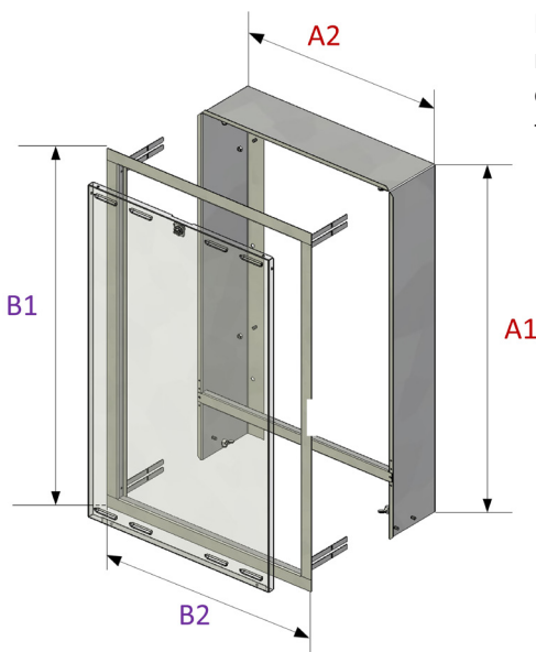
Example representation of the dimensions for UP cladding
