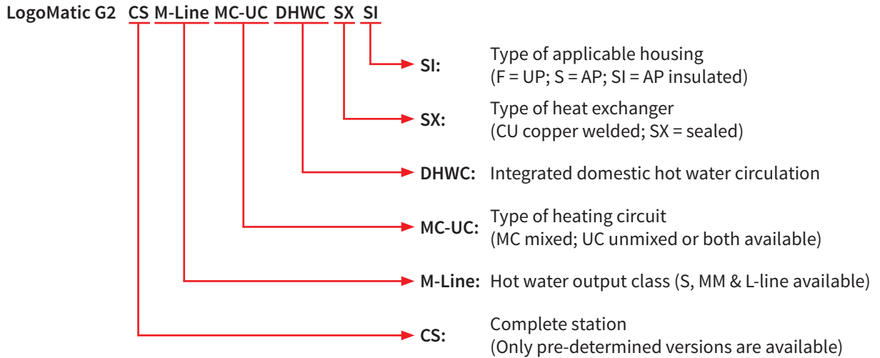
LogoMatic G2 UC DHWC (Unmixed heating circuit as well as domestic hot water circulation)
