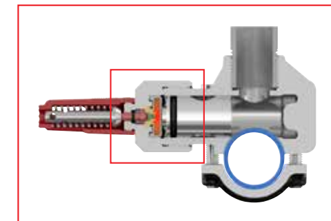
Ignition Once the pin has been removed, the striking pin ignites the charge.
