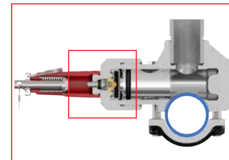
Plunger There is a plunger in the housing of the T-plus.
